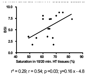
Fig. 2d. 10 and 20-min tissue saturation versus BSI
