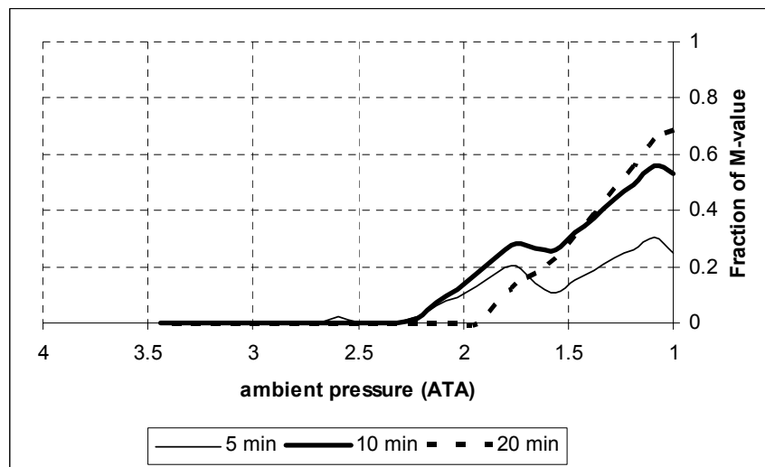
Fig. 4 b. Tracing of predicted tissue saturations for 5, 10 and 20-minute tissues according to the Bühlmann algorithm, vs. fraction of M-value achieved, during decompression from profile 6 (10 m/min ascent rate with deep and shallow stop)
